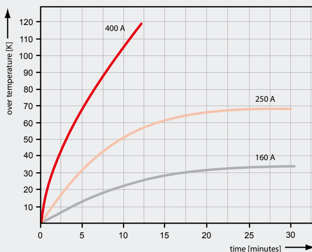
Temperature rise of switching element S307 E and S307 G resp. (wire cross section area 70 mm²)
