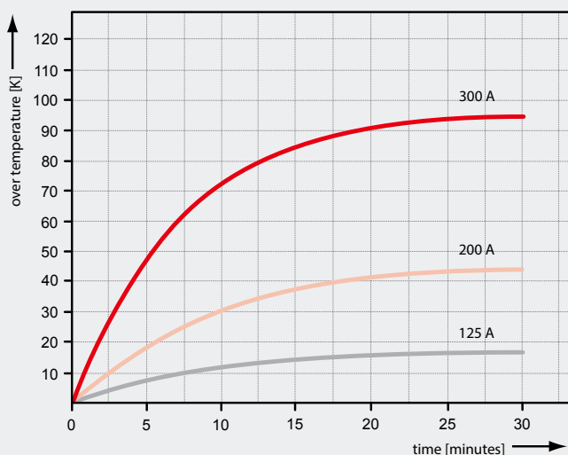
Temperature rise of switching element S306 A and S306 C resp. (wire cross section area 50 mm²)
