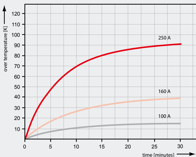
Temperature rise of switching element S306 K and S306 M resp. (wire cross section area 35 mm²)
