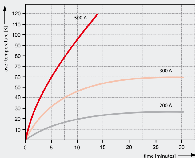
Temperature rise of switching element S307 A and S307 C resp. (wire cross section area 95 mm²)
