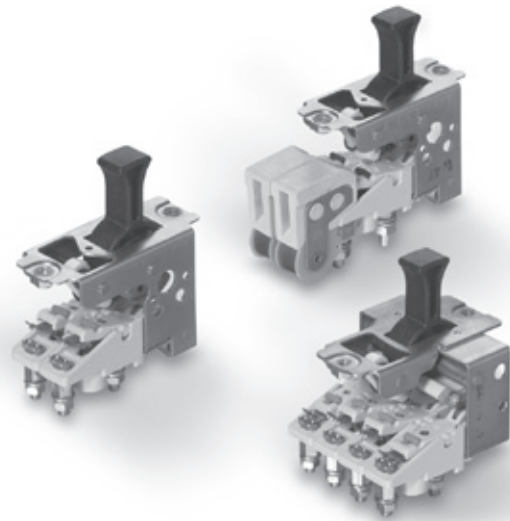
Example: Toggle switch devices with cam-operated switching elements
