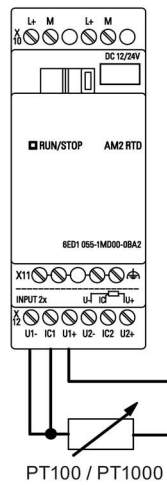
3-wire technique
